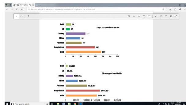
Fig. 2. 2017 Ships scrapped worldwide Source: NGO-Shipbreaking, Platform-stats Graph, (2017)
