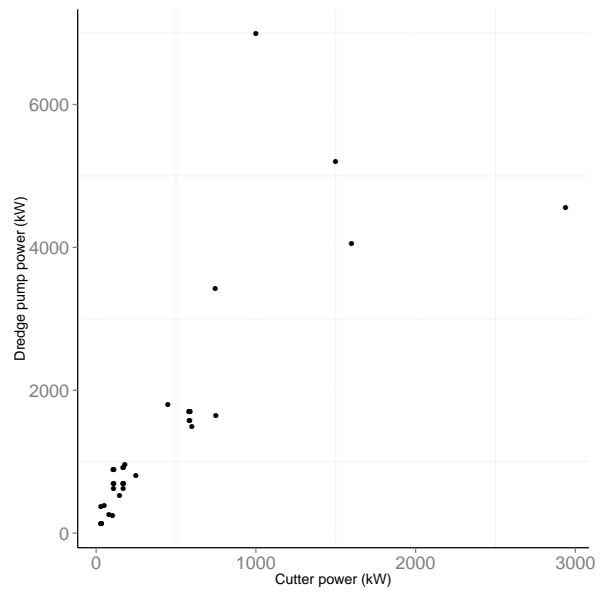
CSD - Cutter power / Dredge pump power
