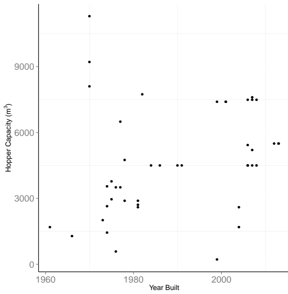
Fig. 4. TSHD - Year Built / Hopper capacity
