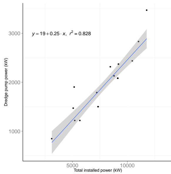
TSHD - Total installed power / Dredge pump power
