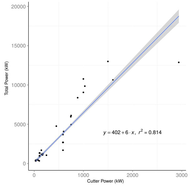
CSD - Cutter power / Total installed power
