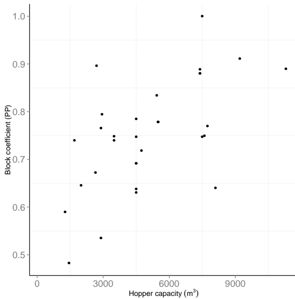
Fig. 3. TSHD - Hopper capacity / C_B (PP)
