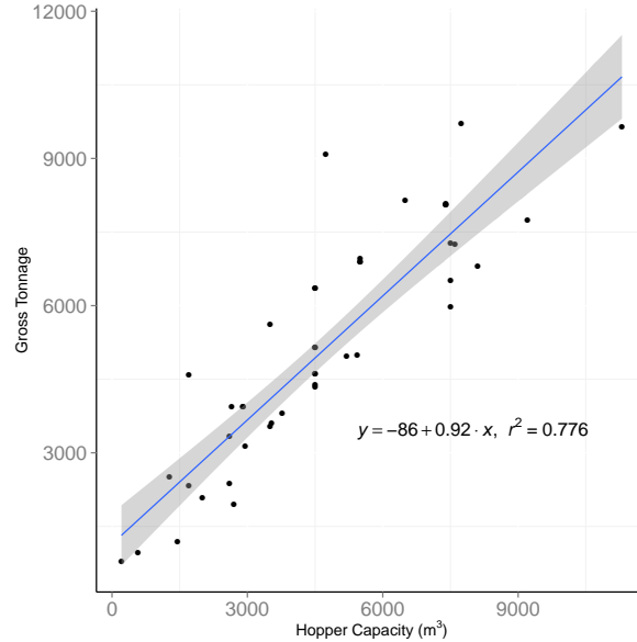
TSHD - Hopper capacity / Gross Tonnage
