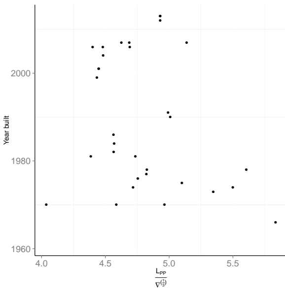
Fig. 5. TSHD - \frac{L_{PP}}{\nabla^{\frac{1}{3}}} / \text{Year Built}
