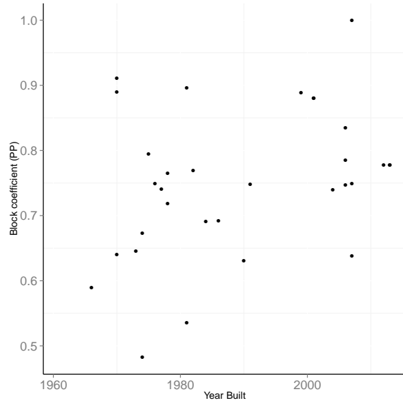
TSHD - Year Built / C_B (PP)
