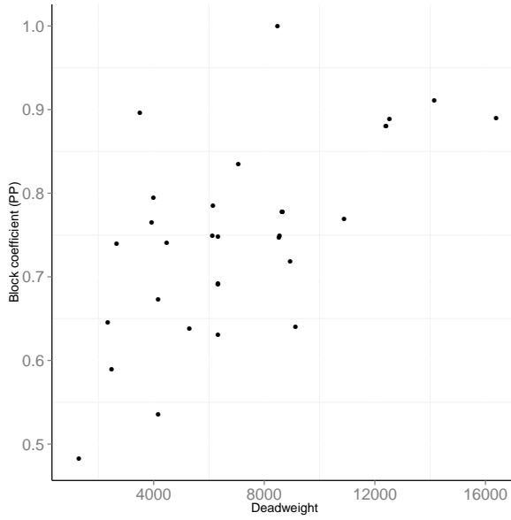
Fig. 2. TSHD - DWT / C_B (PP)
