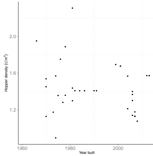
Fig. 6. TSHD - Year Built / Hopper density ( \frac{t}{m^3} )
