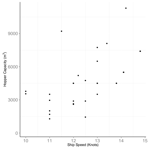
TSHD - Speed / Hopper capacity
