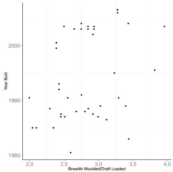
TSHD - Breadth Moulded / Draft Loaded - Year Built
