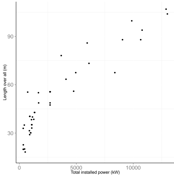
Fig. 8. CSD - Total installed power / Length overall
