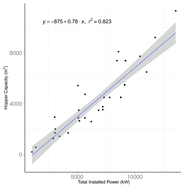
Fig. 7. TSHD - Total installed power / Hopper capacity
