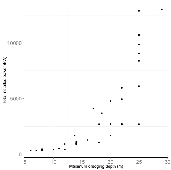
Fig. 9. CSD - Maximum dredging depth / Total installed power
