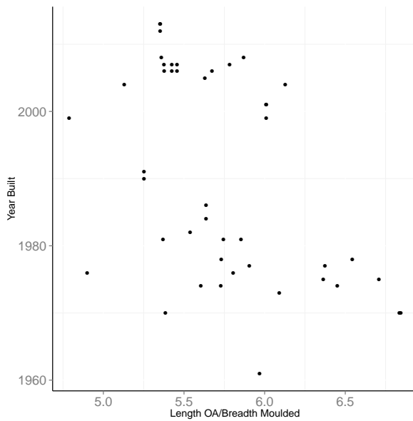
Fig. 1. TSHD - Length OA / Breadth Moulded - Year Built
