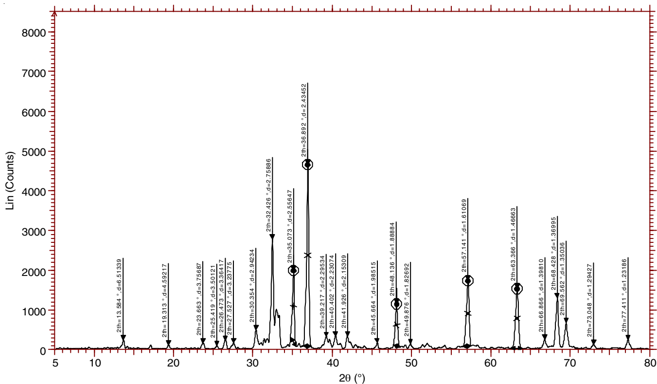
Fig 2. XRD pattern of heterogeneous catalyst at 600 °C
